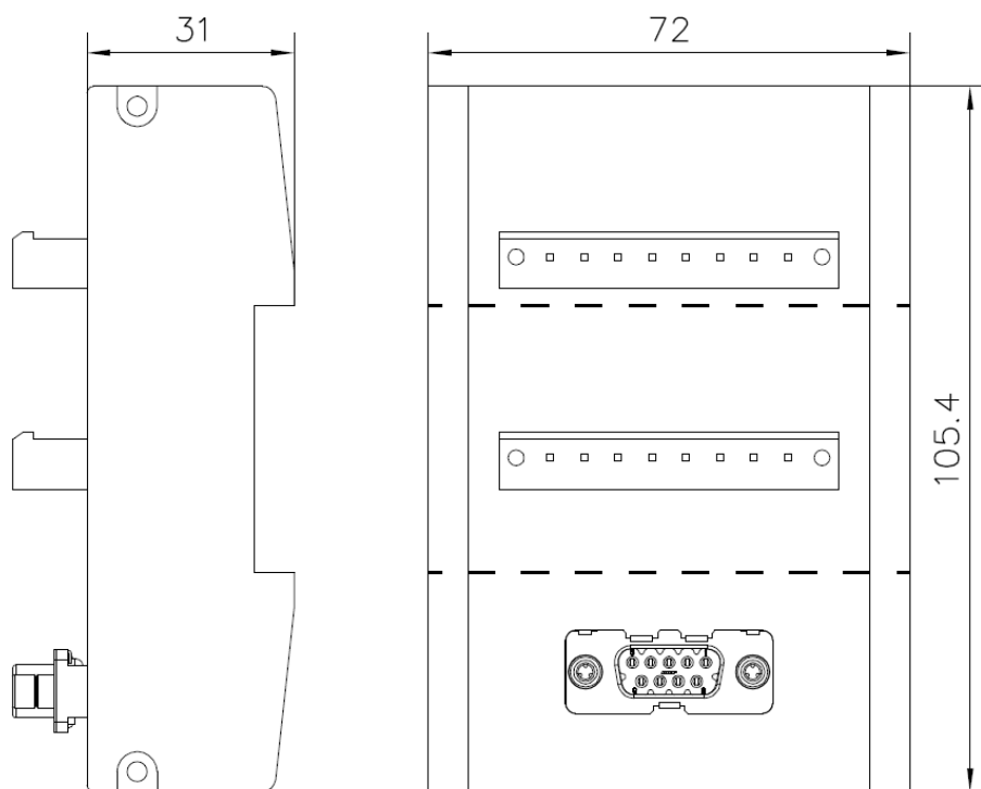
Figure 1: Mechanical dimensions
