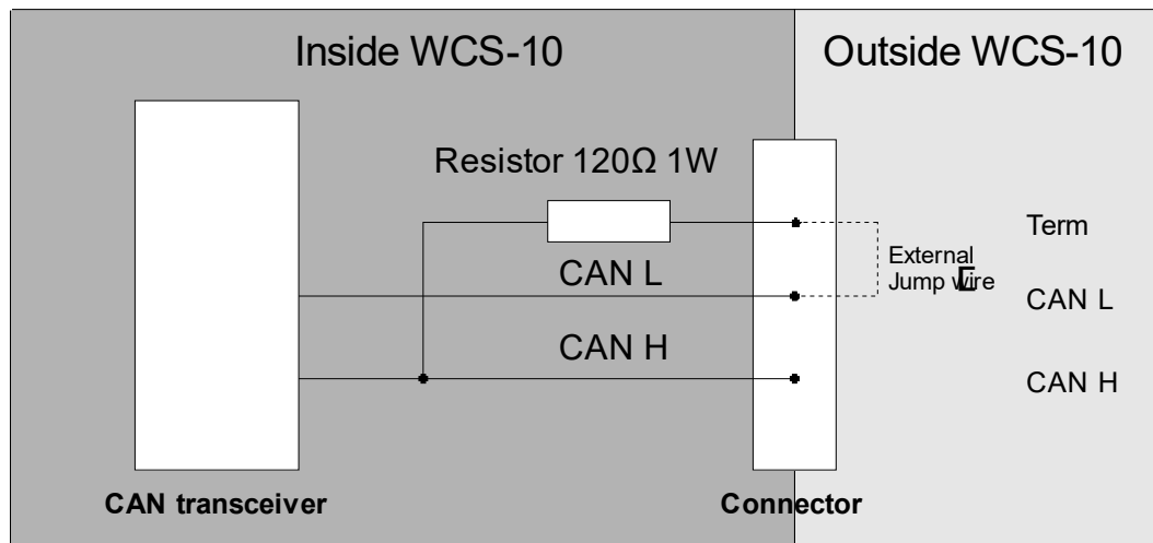
Figure 4: Internal termination
